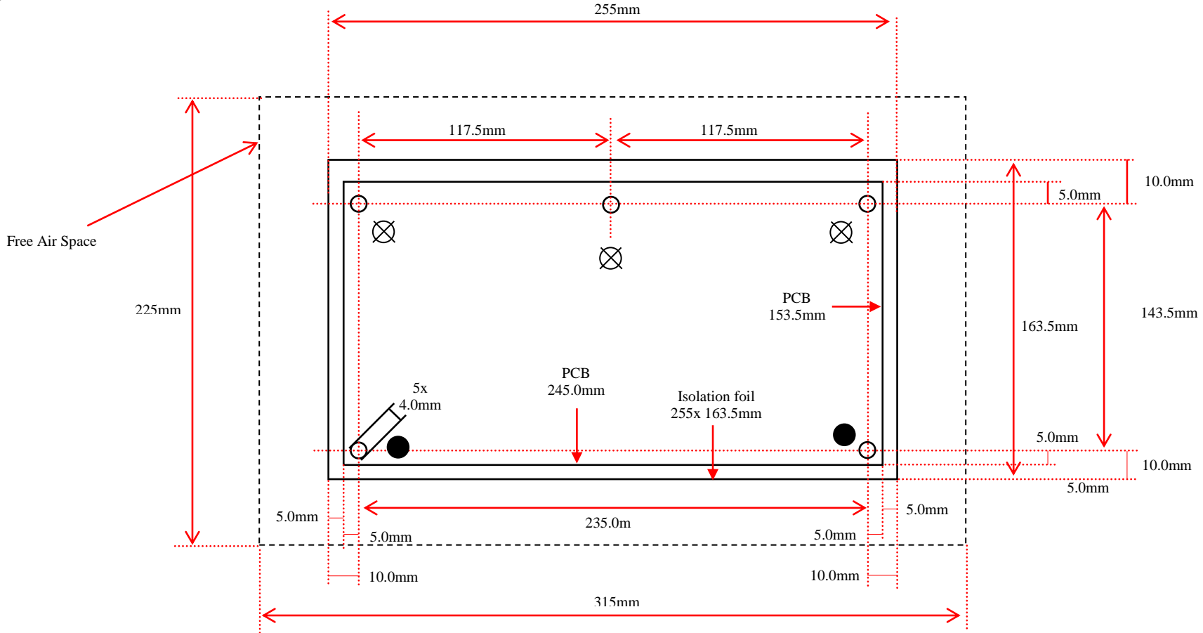
Fig. 7.1.2 SST360i-S mounting holes
